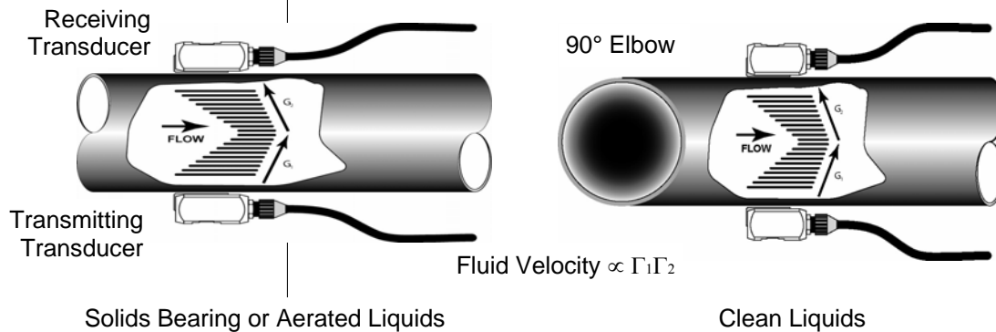
Figure 1 Transducer Locations
